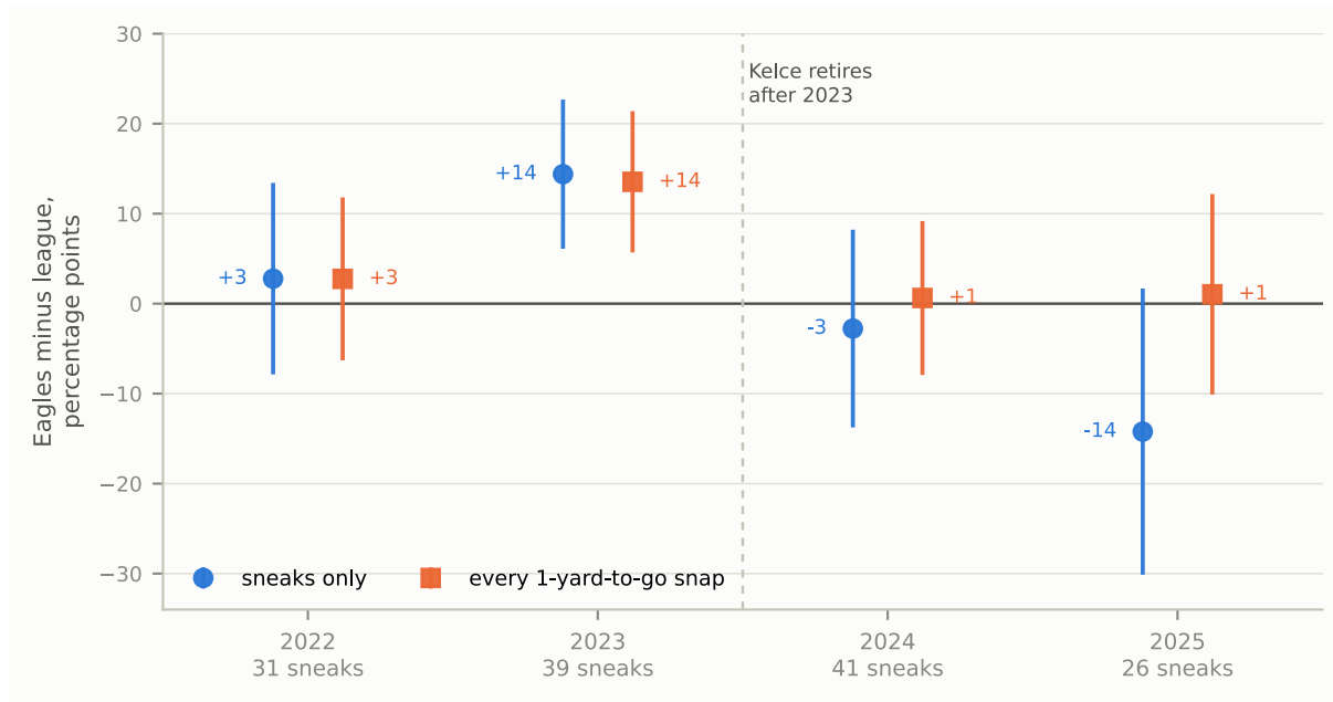
Figure 4: The tush push as an edge: Eagles minus the rest of the league, in percentage points of conversions (first down or touchdown) on 1 yard to go, 2022–2025 regular seasons, with 90% intervals. Blue: quarterback sneaks only (the push and the plain sneak; FTN’s is qb_sneak ). Orange: every snap on 1 yard to go, whatever the call, which removes the question of which plays a team chose to sneak on. Only 2023 stands clearly above zero on either measure; by 2025 the Eagles’ sneaks converted less often than the league’s. The labels under each season give the Eagles’ number of sneaks. Data: nflverse play-by-play joined to FTN charting.
