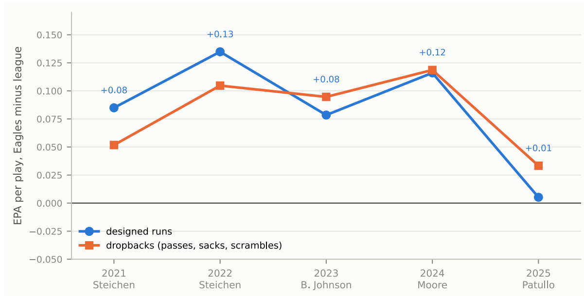
Figure 3: The Eagles’ offense against the league, by season and offensive coordinator, 2021–2025 regular seasons: expected points added (EPA) per play on designed runs and on dropbacks, minus the league average (above zero is better than average). The run game stayed well above average under three different coordinators, and the passing game rose with it, until both fell back toward average in 2025. Data: nflverse play-by-play (runs exclude quarterback scrambles, which count as dropbacks).
