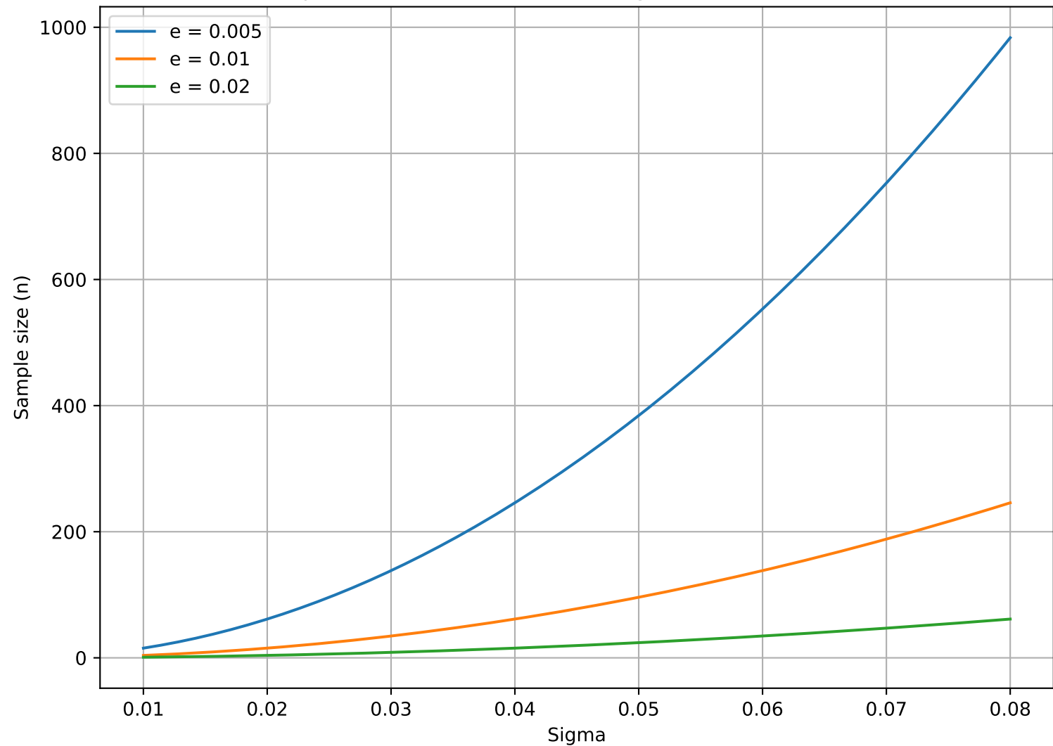
Sample size (n) as a function of sigma at 95% confidence
