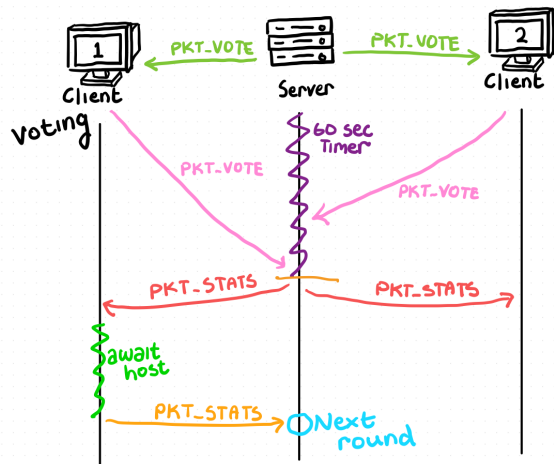
Figure 3: Architecture diagram for voting
