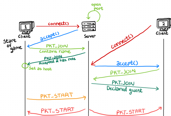
Figure 1: Architecture diagram for starting the game
