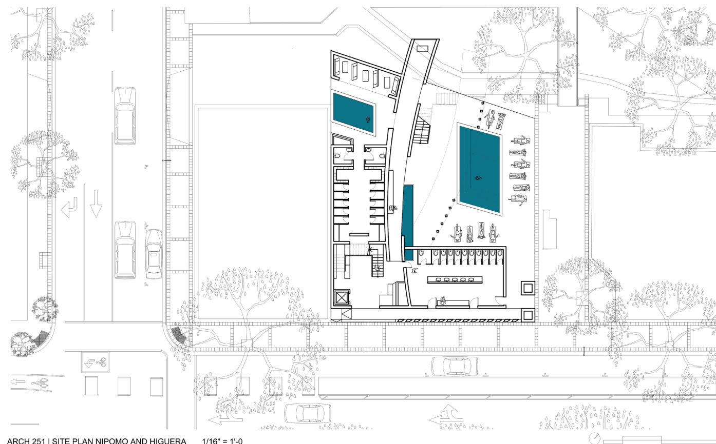
ARCH 251 | SITE PLAN NIPOMO AND HIGUERA 1/16" = 1'-0
