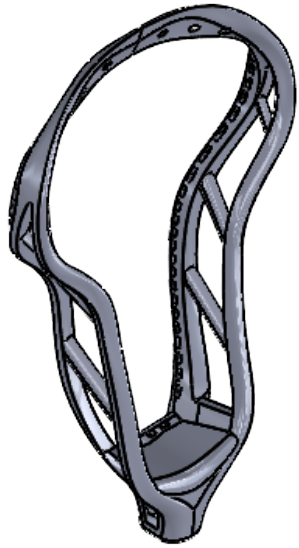
Shooter Head v9 Isometric View
