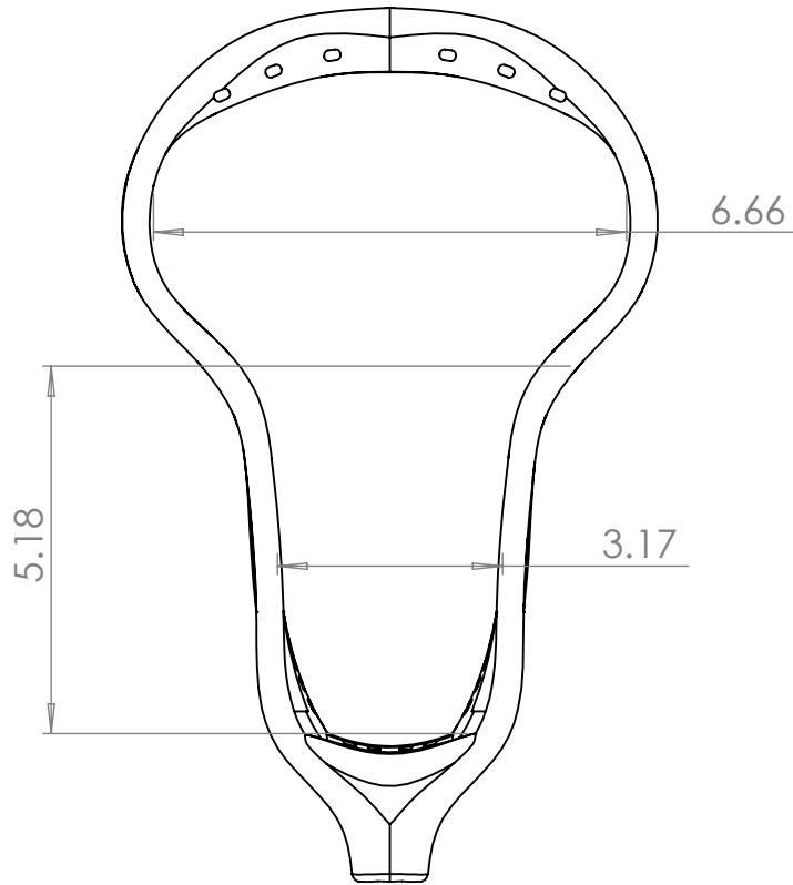
Shooter Head v9 Front View Nylon
