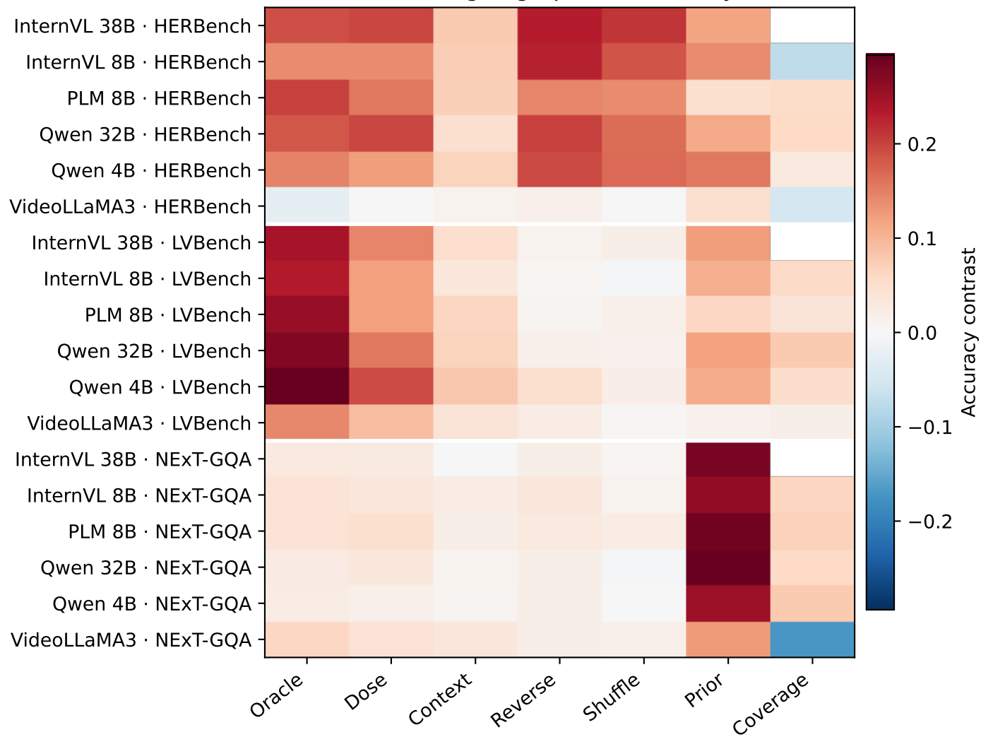
Evaluation-setting fingerprints (accuracy contrast)
