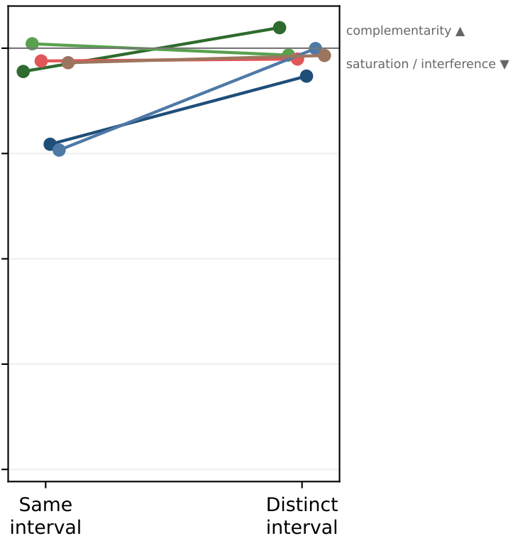
HERBench
