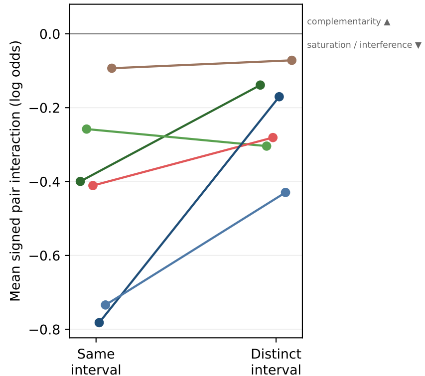
NExT-GQA
