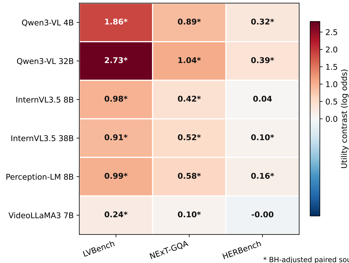
Individual evidence utility (17/18 settings ↑) Evidence minus matched outside frames
