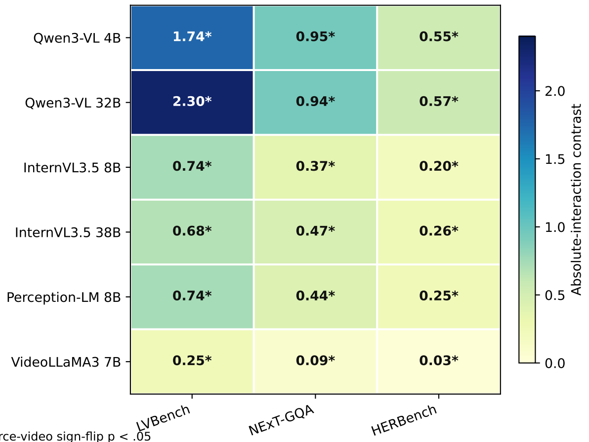
Pairwise non-additivity (18/18 settings ↑) Evidence pairs minus outside-frame pairs
