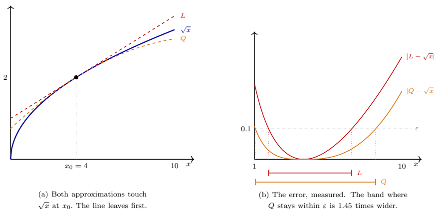
Figure 6.1: Linear and quadratic approximation of the square root at x_0 = 4
