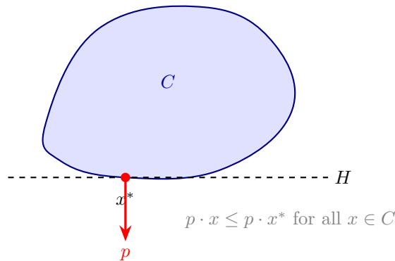
Figure 13.4: Supporting Hyperplane
