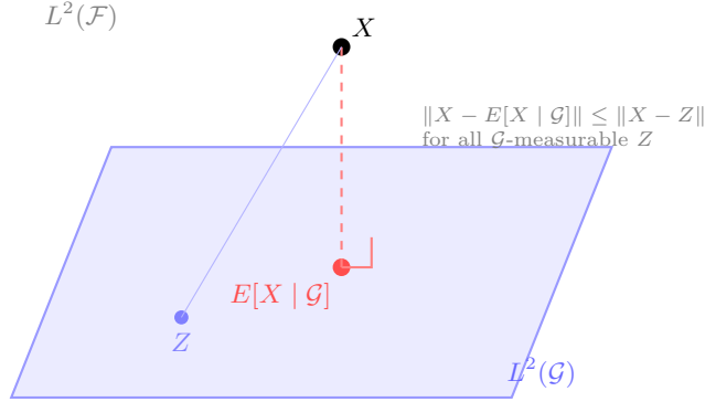
Figure 15.2: Conditional expectation as projection in L^2
