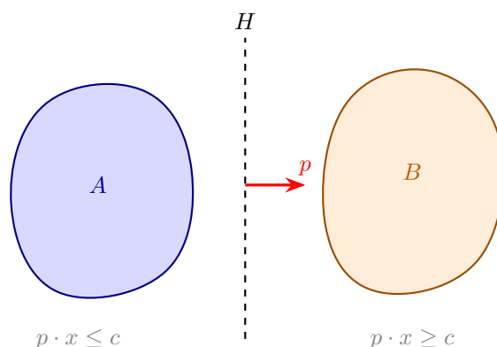
Figure 13.3: Separating Hyperplane
