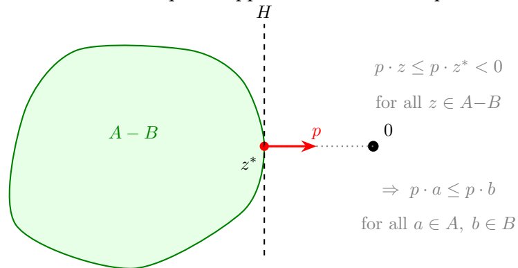
Figure 13.5: Separating from supporting
