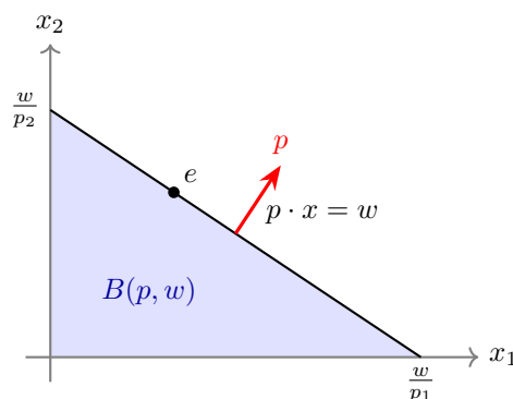
Figure 13.2: Budget Set
