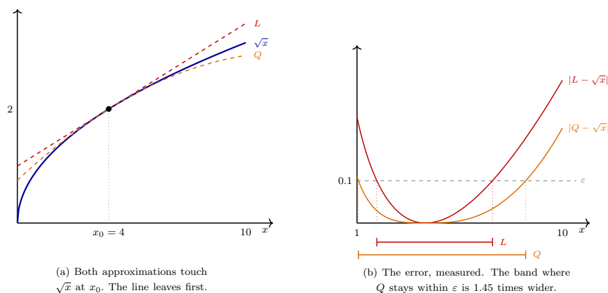
Figure 1: Linear and quadratic approximation of the square root at x_0 = 4
