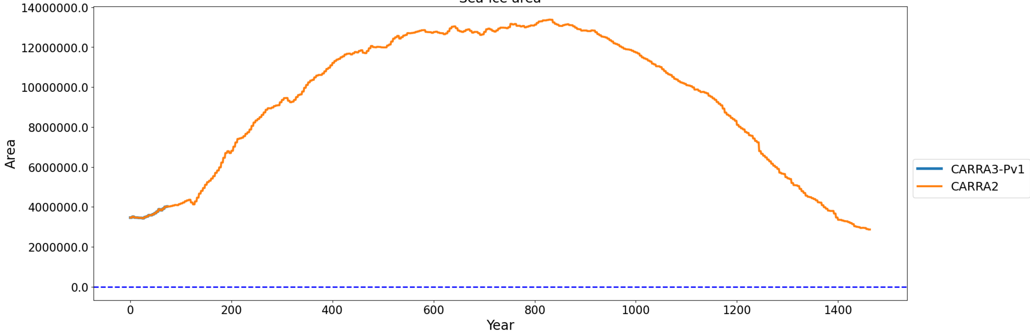
Sea-ice area
