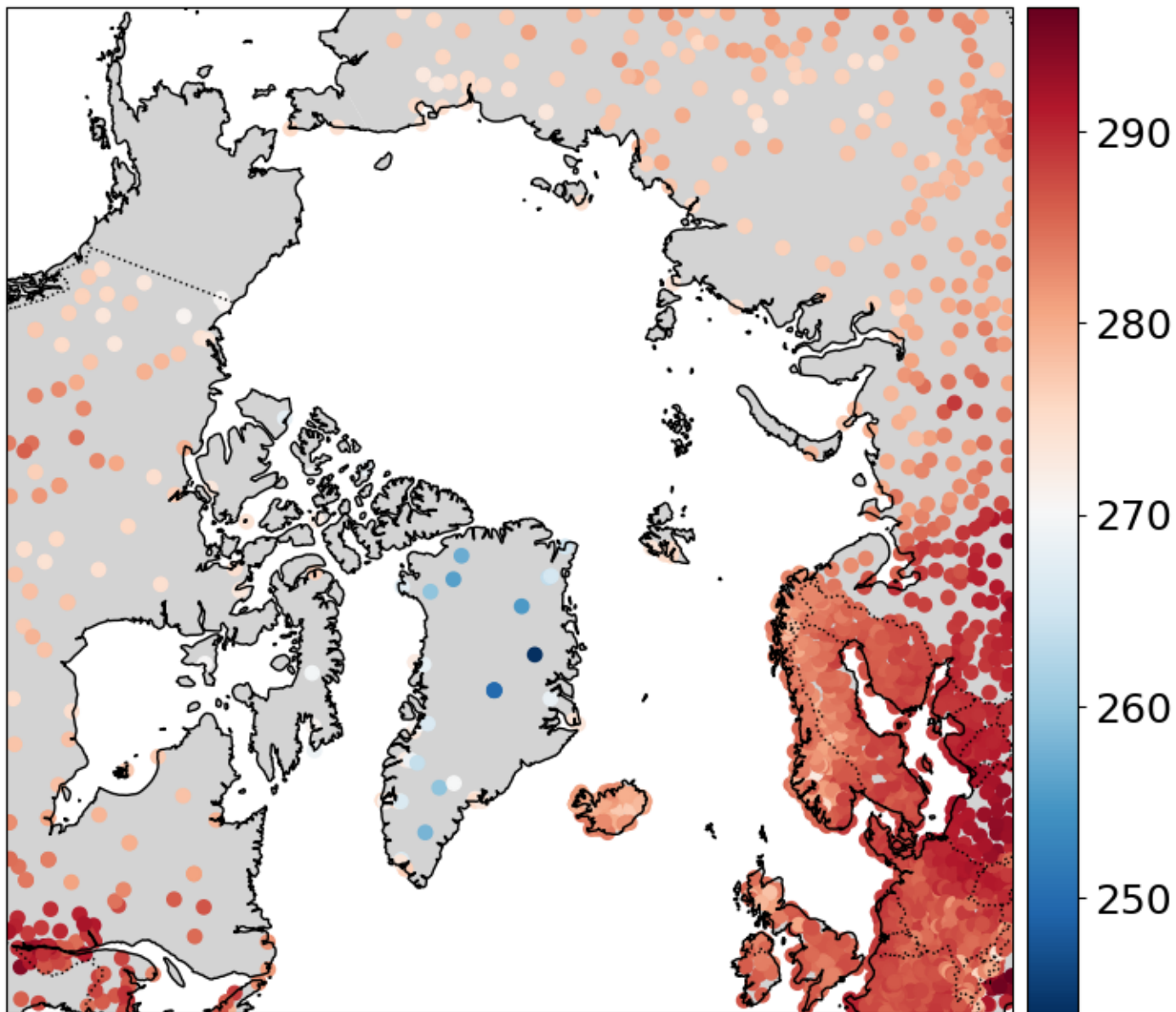
T2M observations
