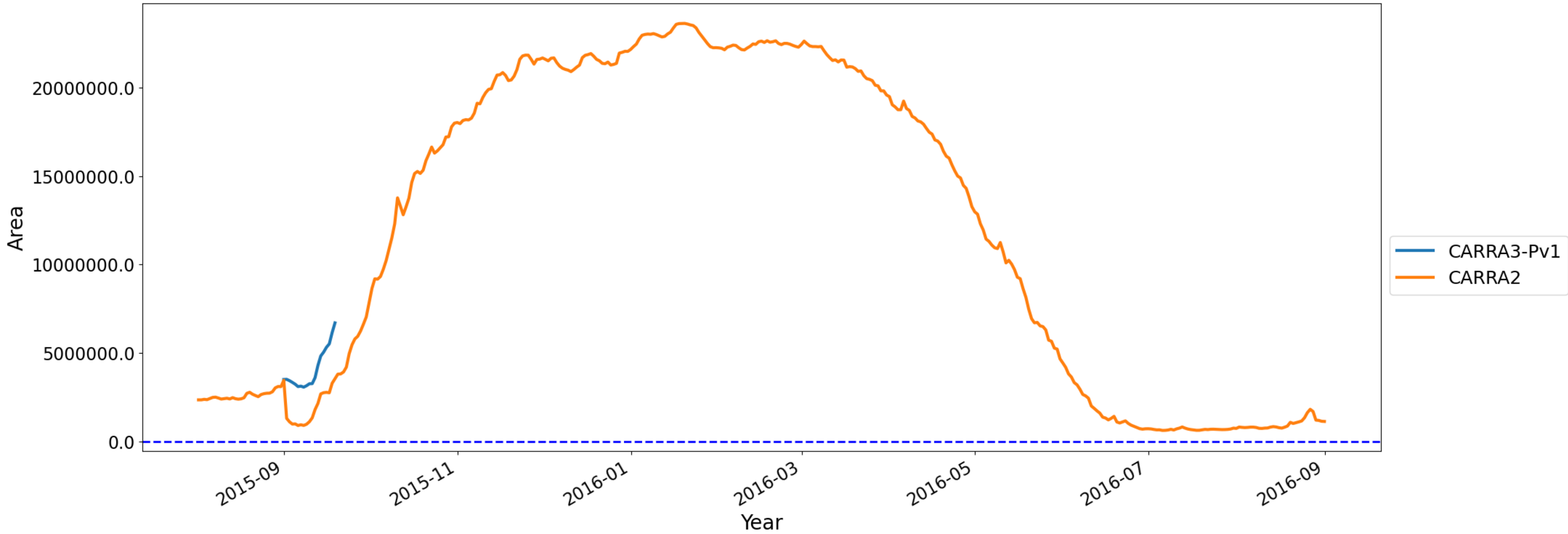
Seasonal snow covered area
