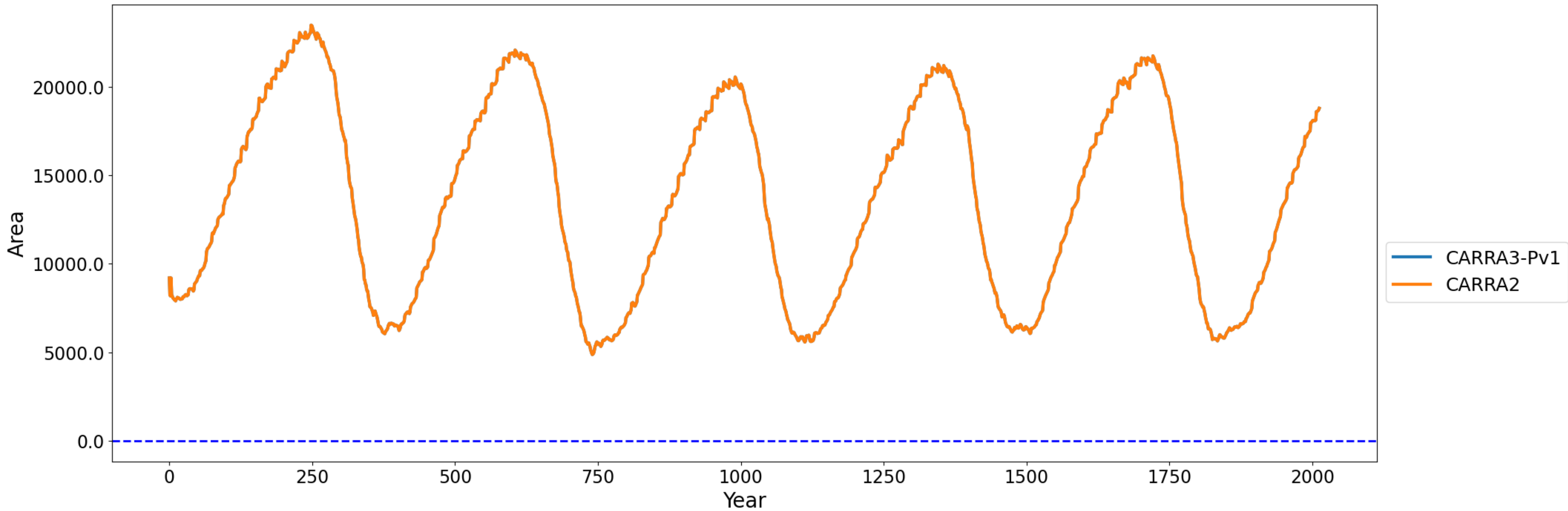
Sea-ice area
