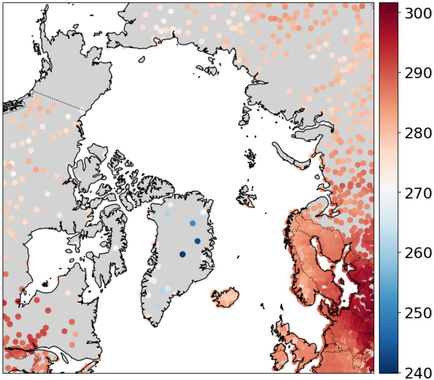
T2M observations
