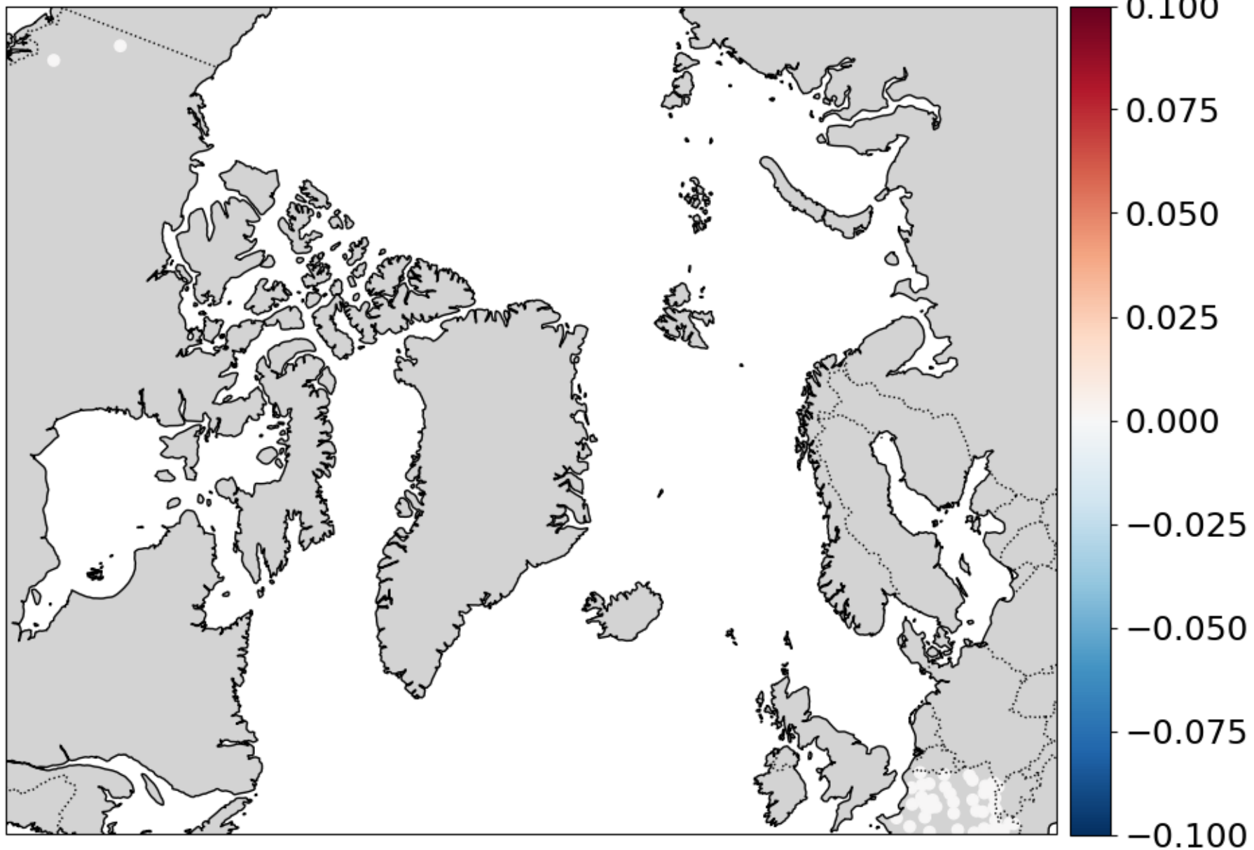
SD observations
