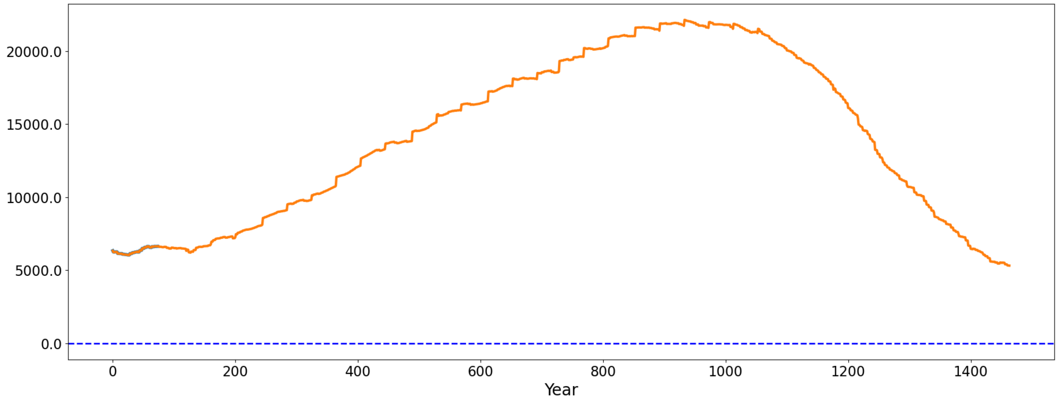
Sea-ice volume
