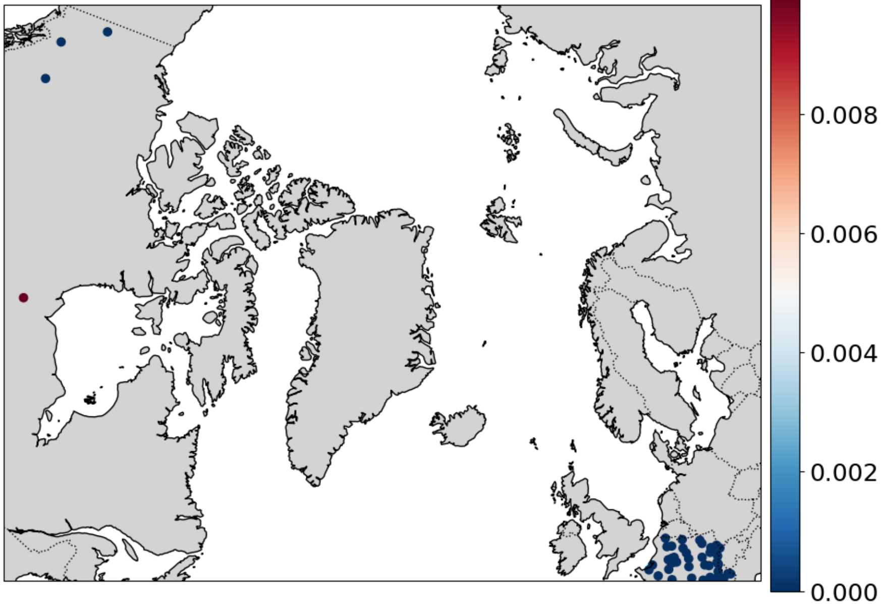
SD observations
