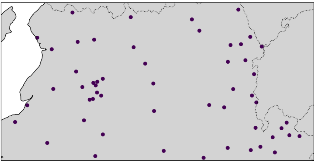
SD observations
