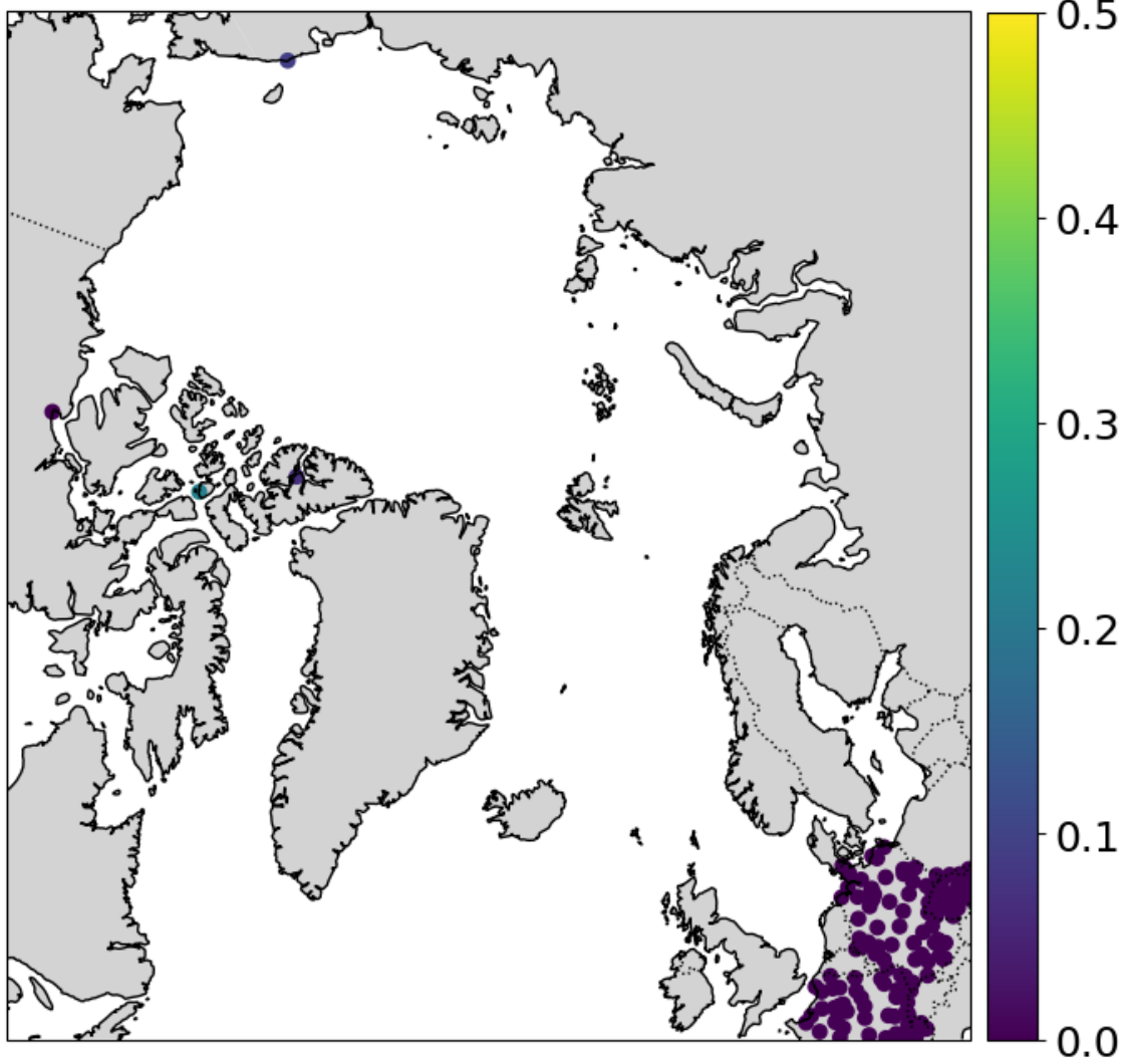
SD observations
