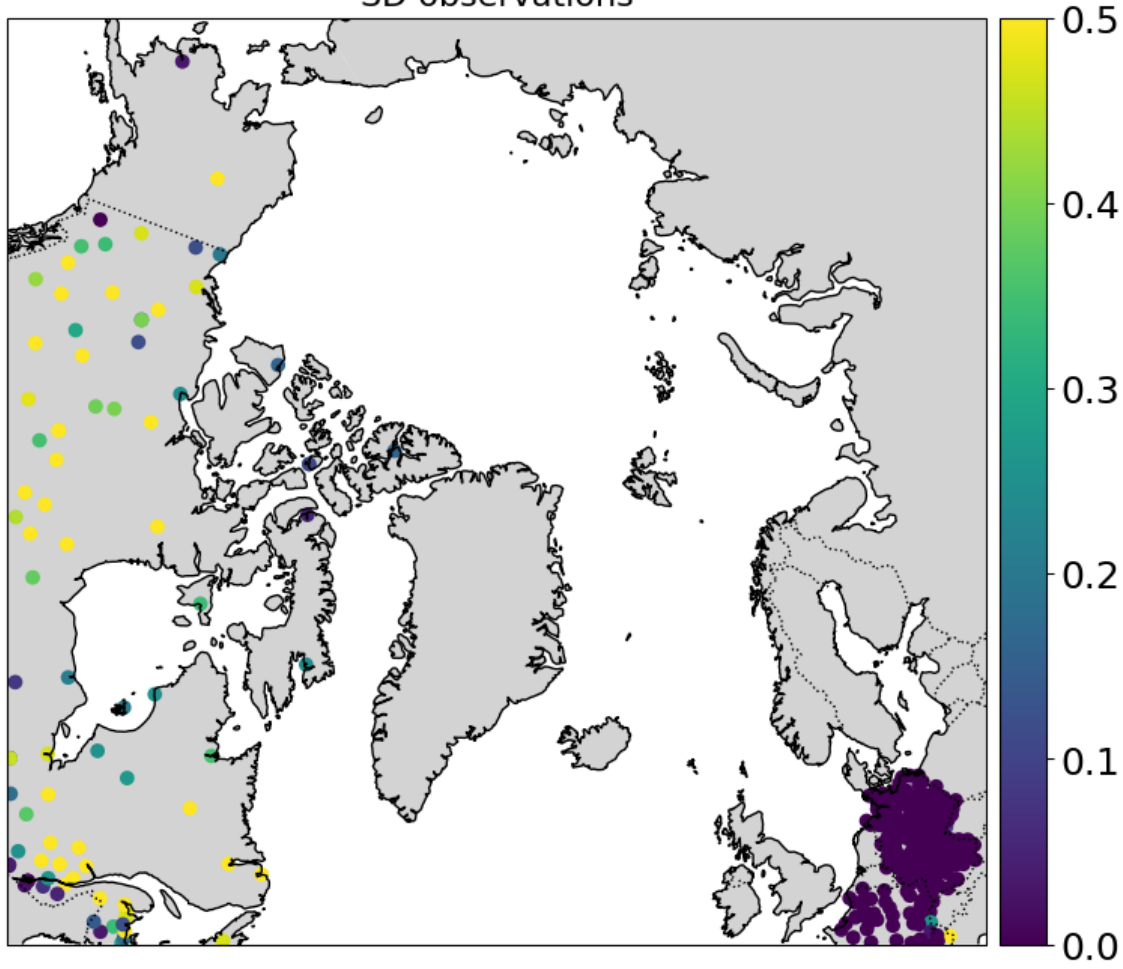
SD observations
