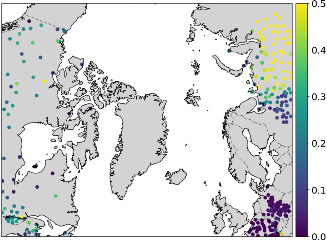
SD observations
