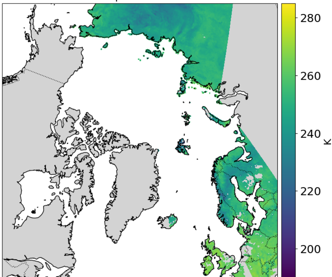
18GHz V-pol Observation
