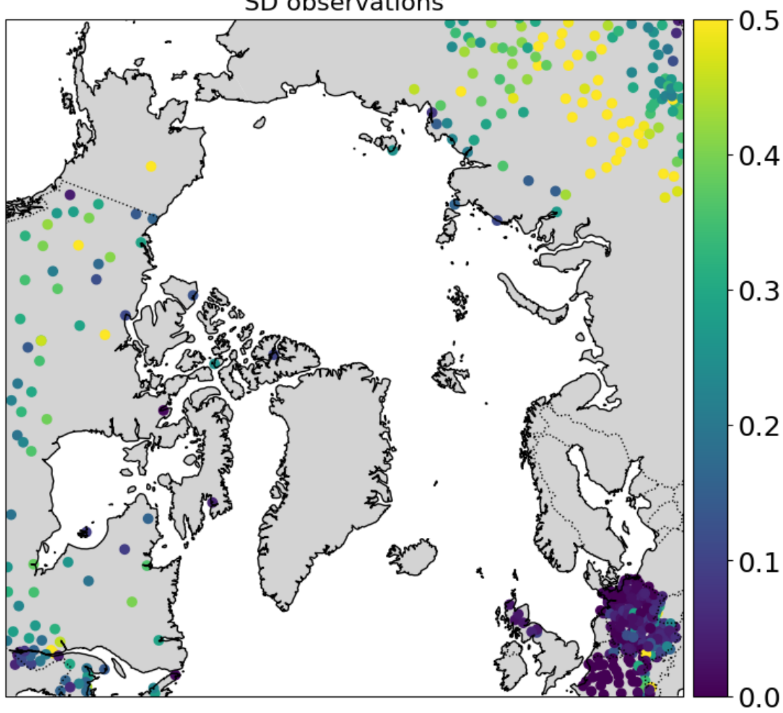
SD observations
