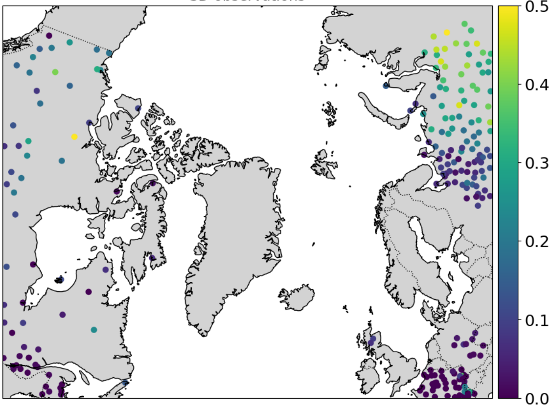
SD observations
