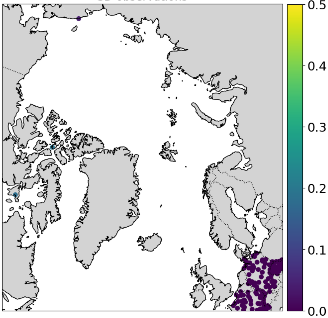
SD observations
