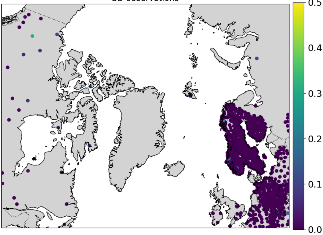
SD observations
