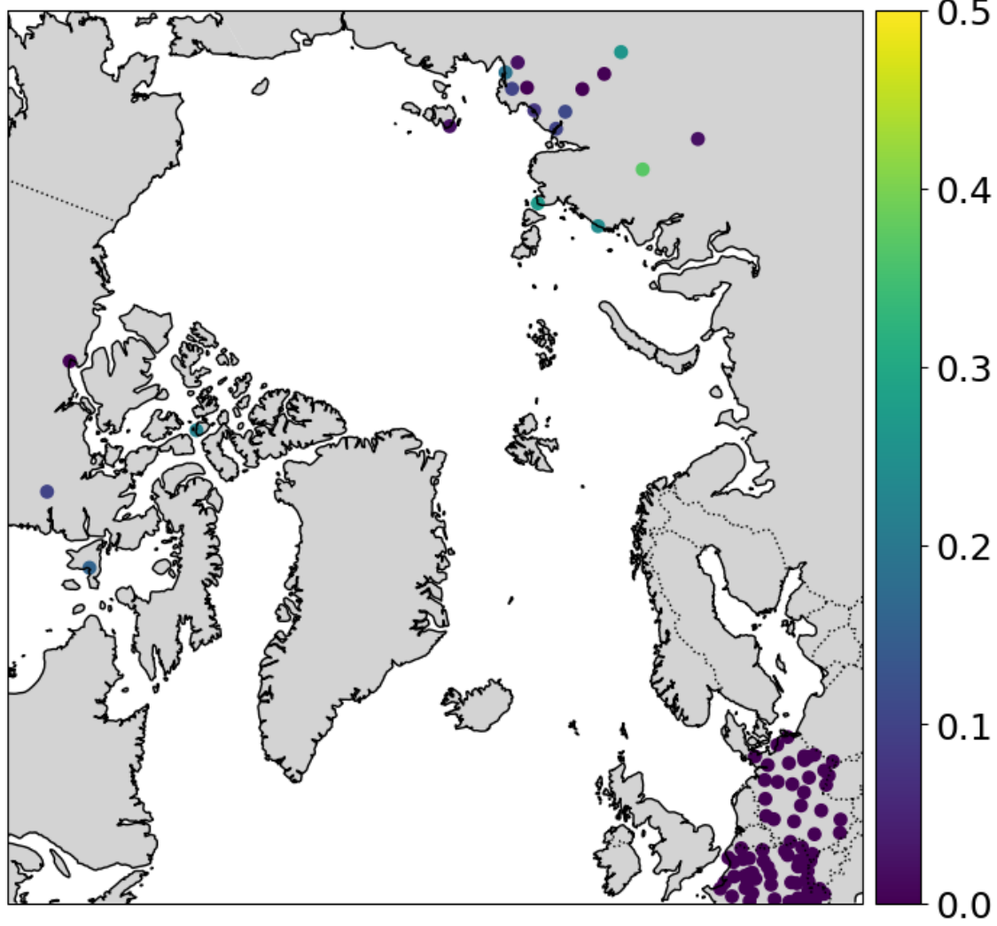
SD observations
