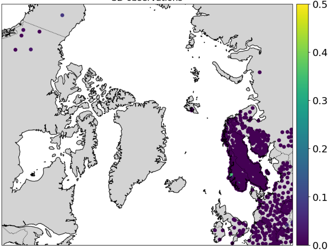
SD observations
