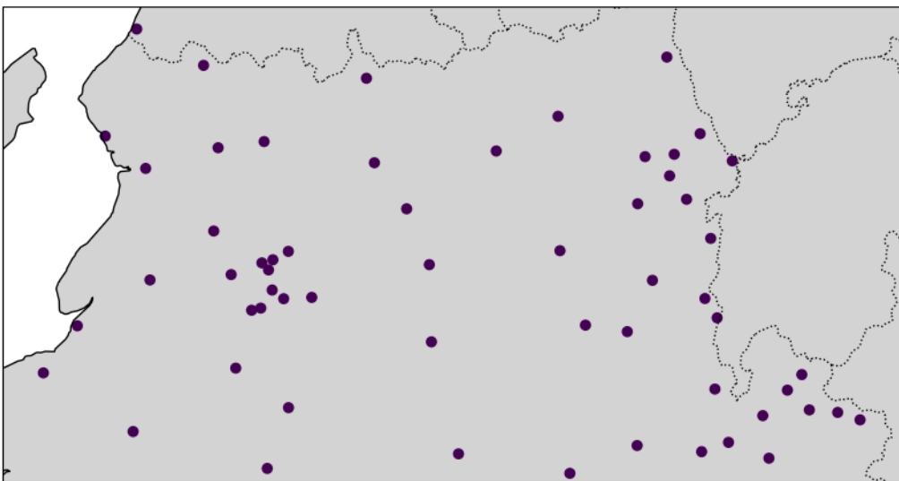
SD observations
