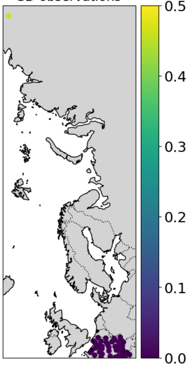
SD observations
