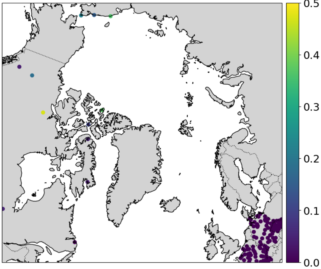
SD observations
