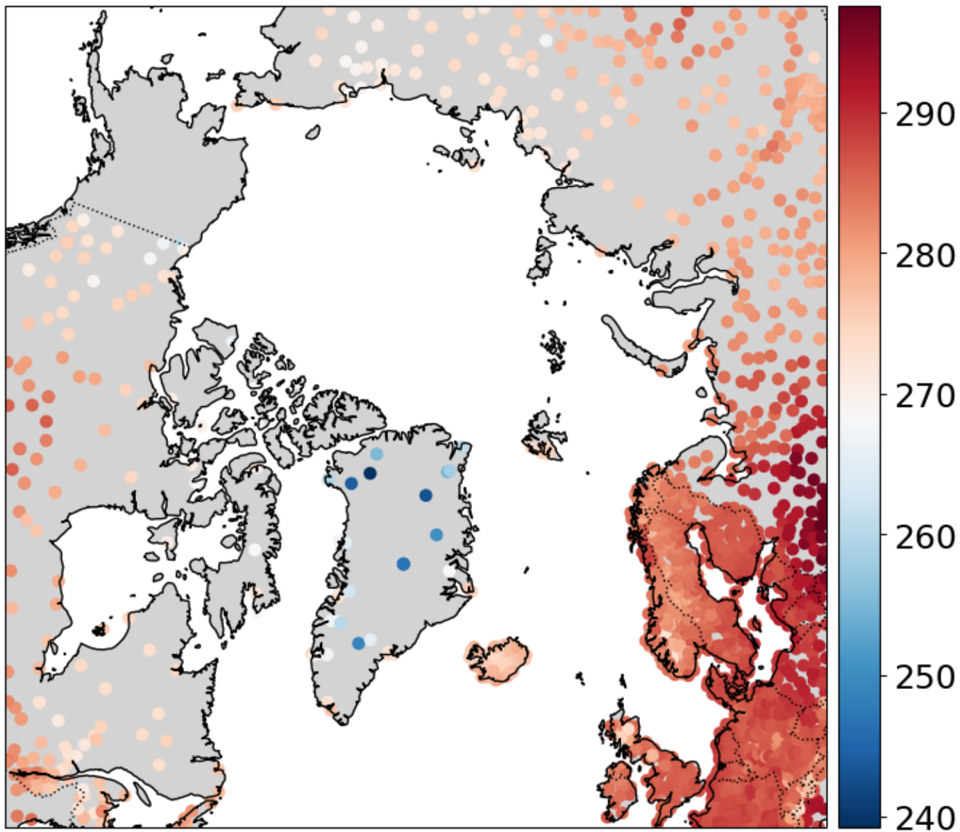
T2M observations
