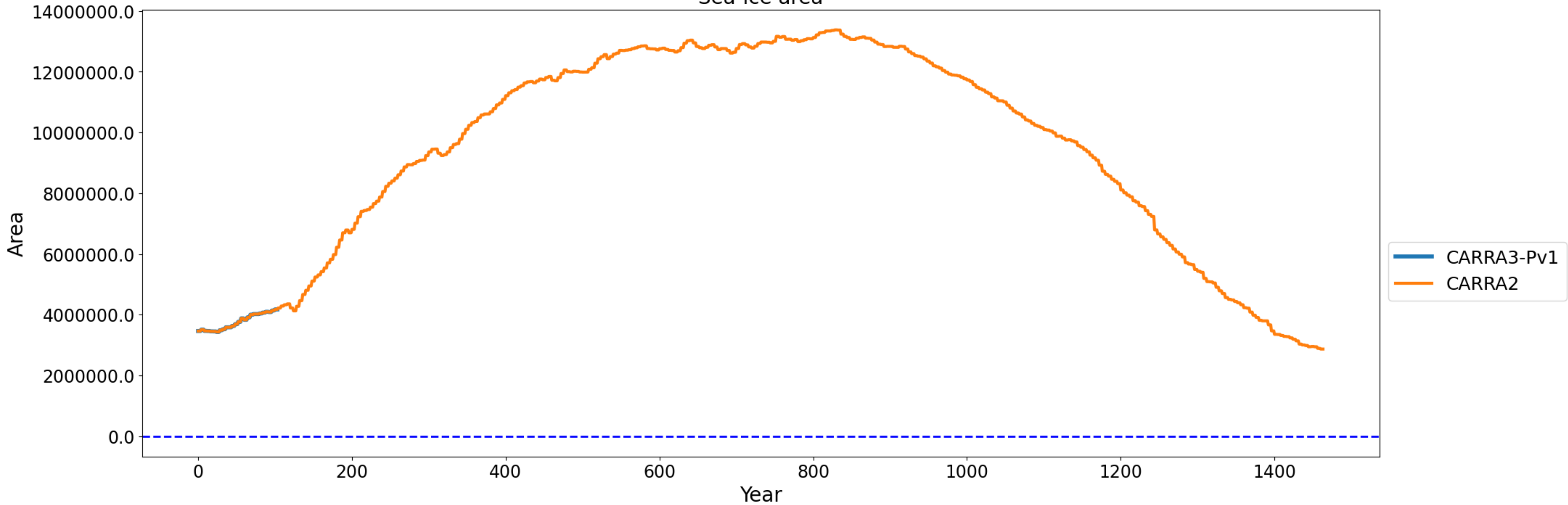
Sea-ice area
