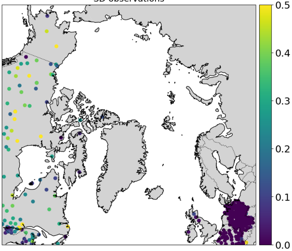
SD observations
