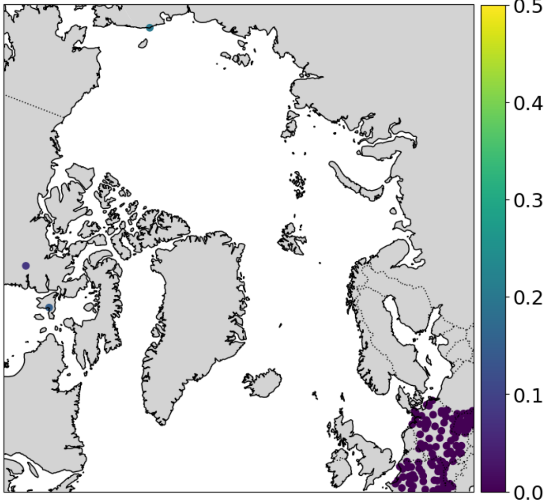
SD observations
