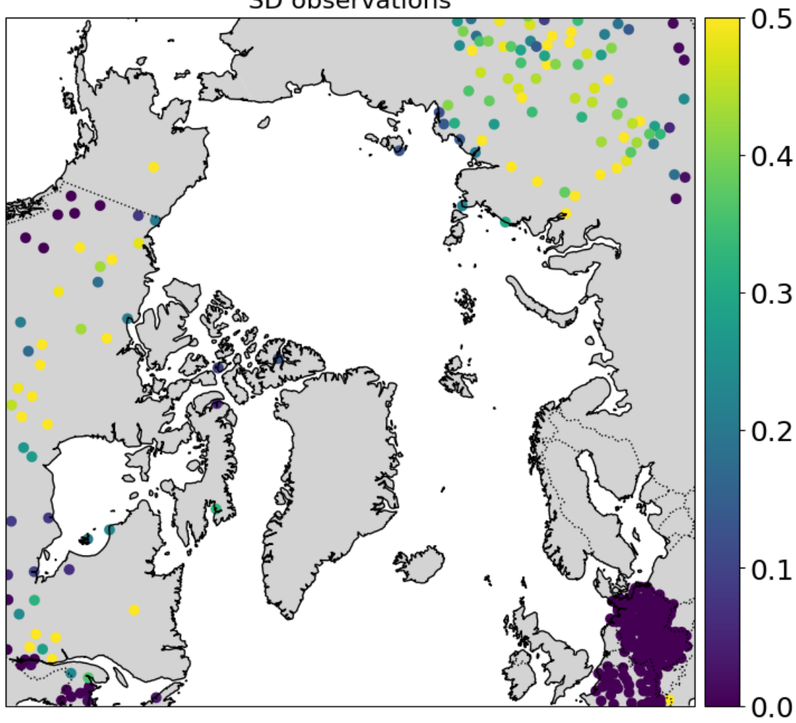
SD observations
