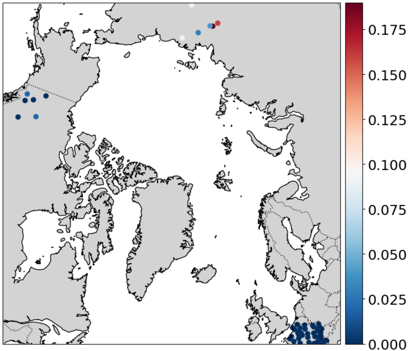
SD observations
