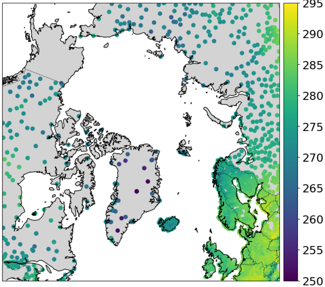
T2M observations
