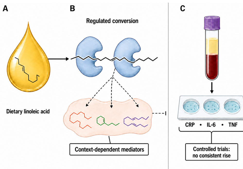
Figure 3. Controlled human trials do not show a consistent systemic inflammatory response. Panel A identifies the dietary linoleic-acid input. Panel B shows multiple regulated processing steps and dashed, context-dependent mediator branches; the dashed path stops at the evidence boundary because possible local signaling does not establish a systemic response. Panel C shows the conventional circulating markers measured in controlled feeding trials—CRP, IL-6, and TNF—which do not rise consistently on average. The figure does not exclude local signaling, susceptible subgroups, or unmeasured long-term outcomes. 40,41,43,44
