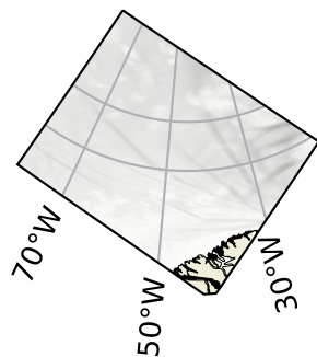
c) SEDNA Ice Concentration
