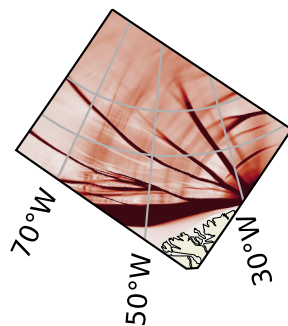
d) SEDNA Total deformation
