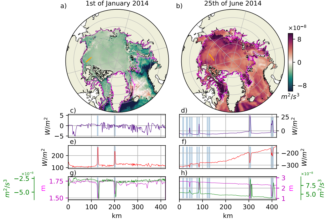
Figure 2. Maps of buoyancy flux and transects for the 1st of January and 25th of June 2014.
