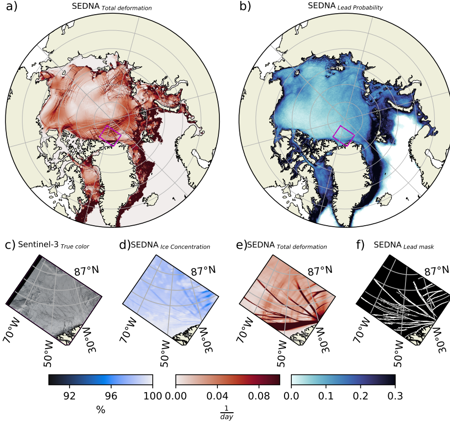
Figure 1. Linear kinematic features from SEDNA. a) Snapshot of the total deformation for the 21st of April 2014. b) Linear kinematic mean frequency between 2011 and 2015. c) True color image from Sentinel 3 on the 12th of April 2022 for the magenta area in panel a. d) Mean ice concentration from SEDNA on the 21st of April 2014. e) Total deformation used to identifies the linear kinematic features. f) Identified linear kinematic features on the 21st of April 2014.
