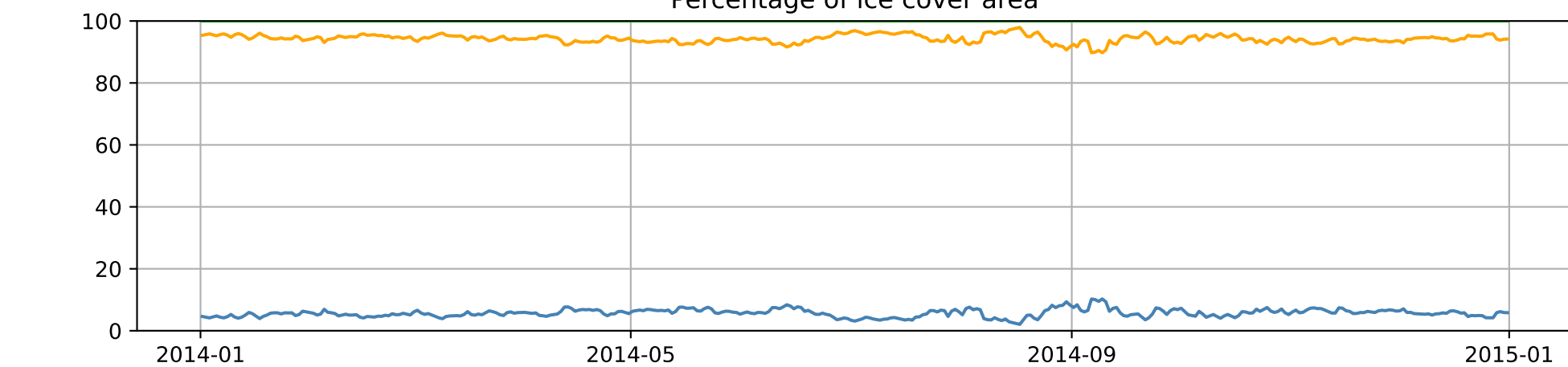
Percentage of ice cover area
