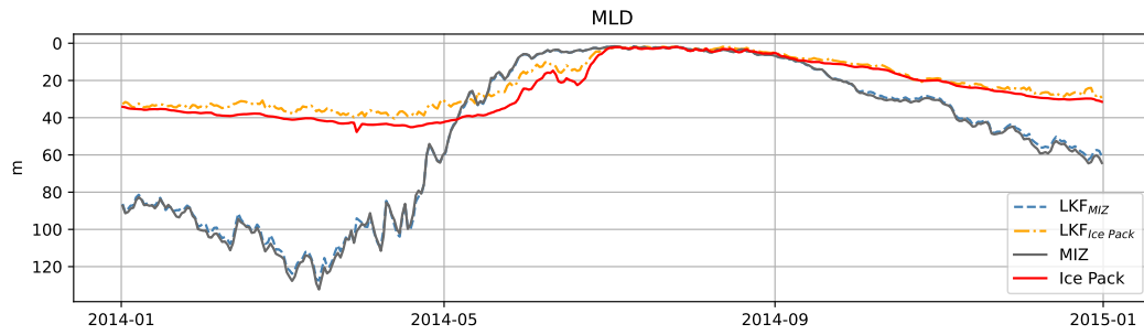
Figure S2. Time-series during 2014 of the mean mixed layer depth for linear kinematic features in the ice pack, the linear kinematic features in the marginal ice zone, the marginal ice zone (ice concentration 0-80%), and the ice pack (ice concentration \geq 80\% ).
