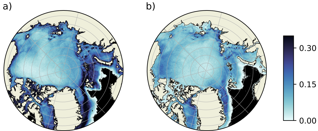
Figure S1. Linear kinematic mean frequency from a) SEDNA and b) Thermal-Infrared Satellite Imagery (Willmes et al., 2023) between 2011 and 2015 TODO: Add contours of KE and topography
