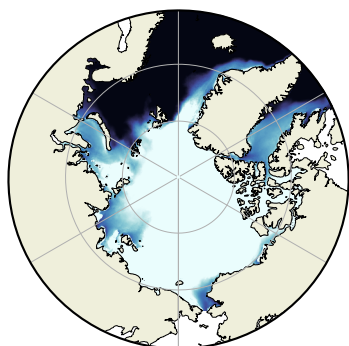
c) SEDNA: temperature at 5m depth
