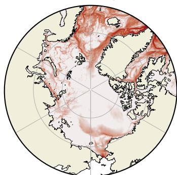
h) CREG: kinetic energy at 5m depth
