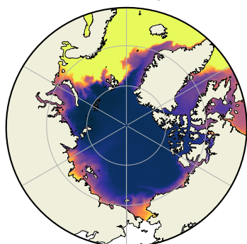
f) CREG: salinity at 5m depth
