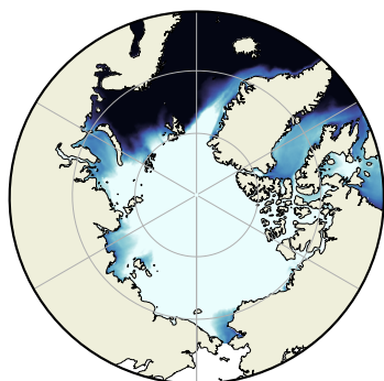
d) CREG: temperature at 5m depth
