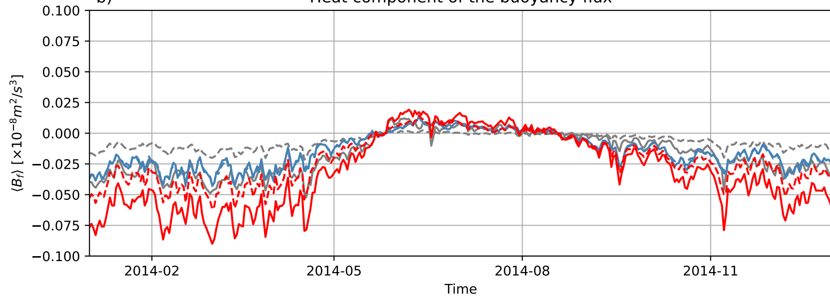
Heat component of the buoyancy flux
