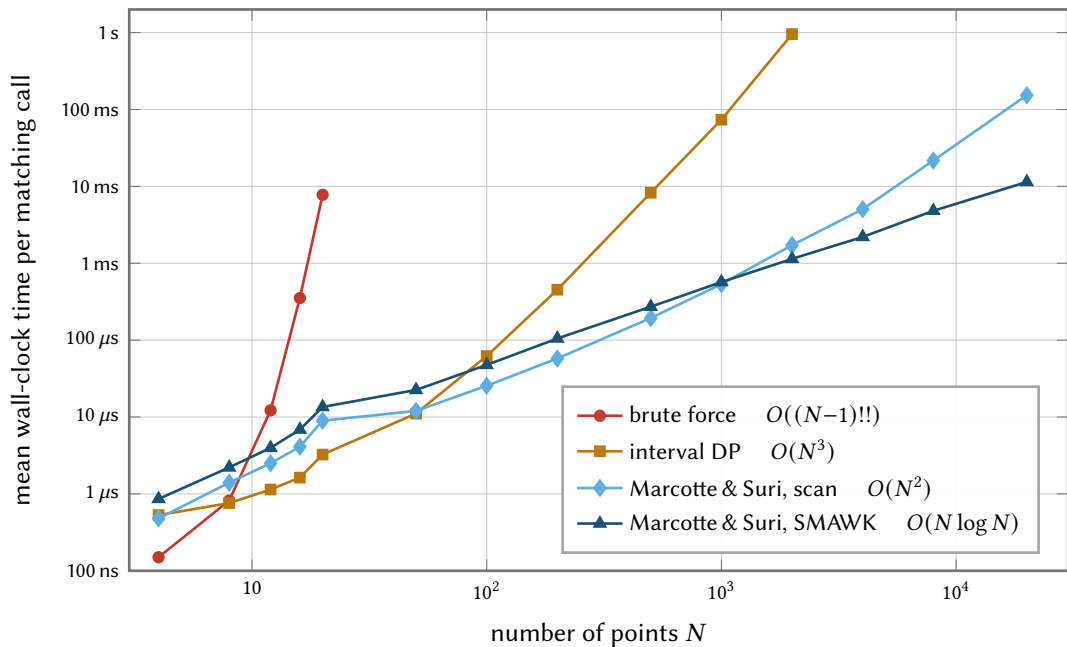
Minimum-weight non-crossing matching: time vs. input size
