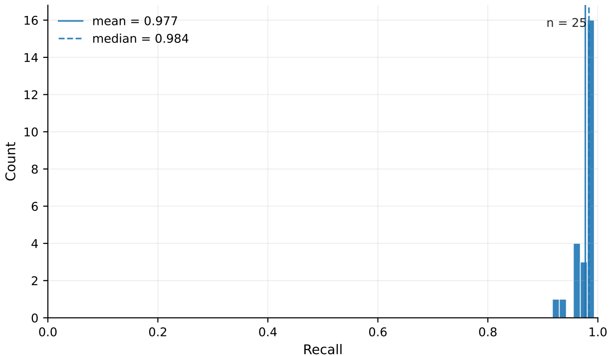
Recall distribution
