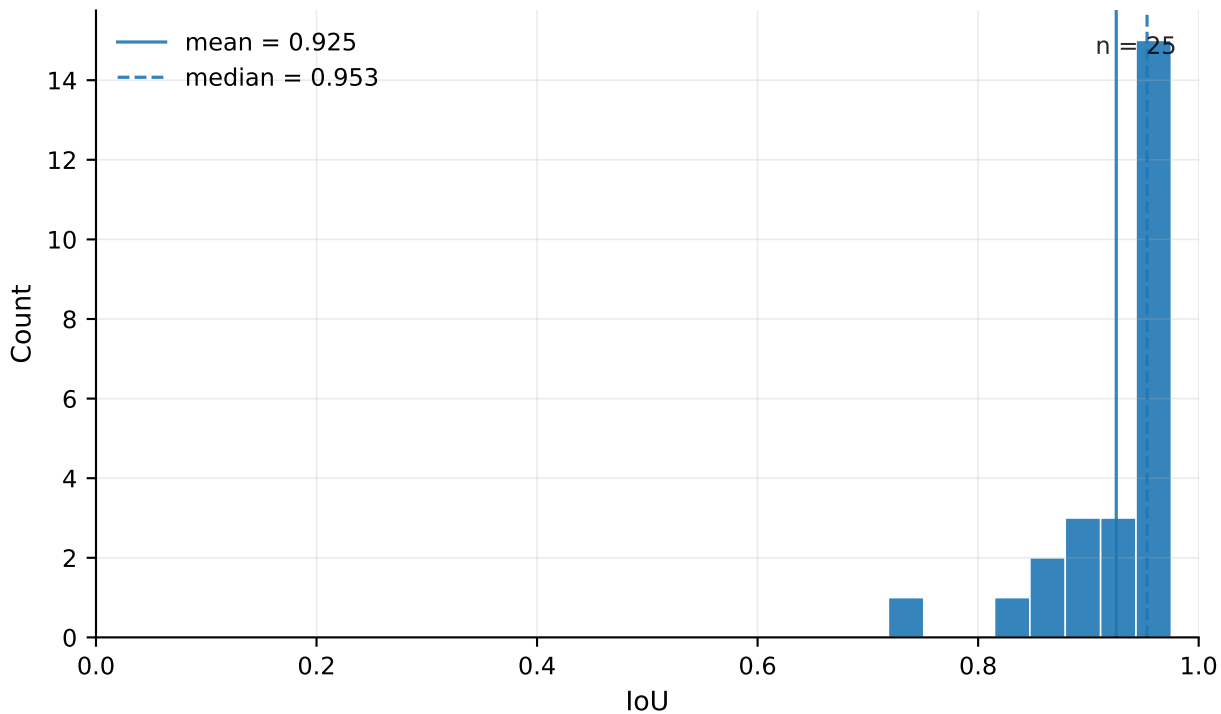
IoU distribution
