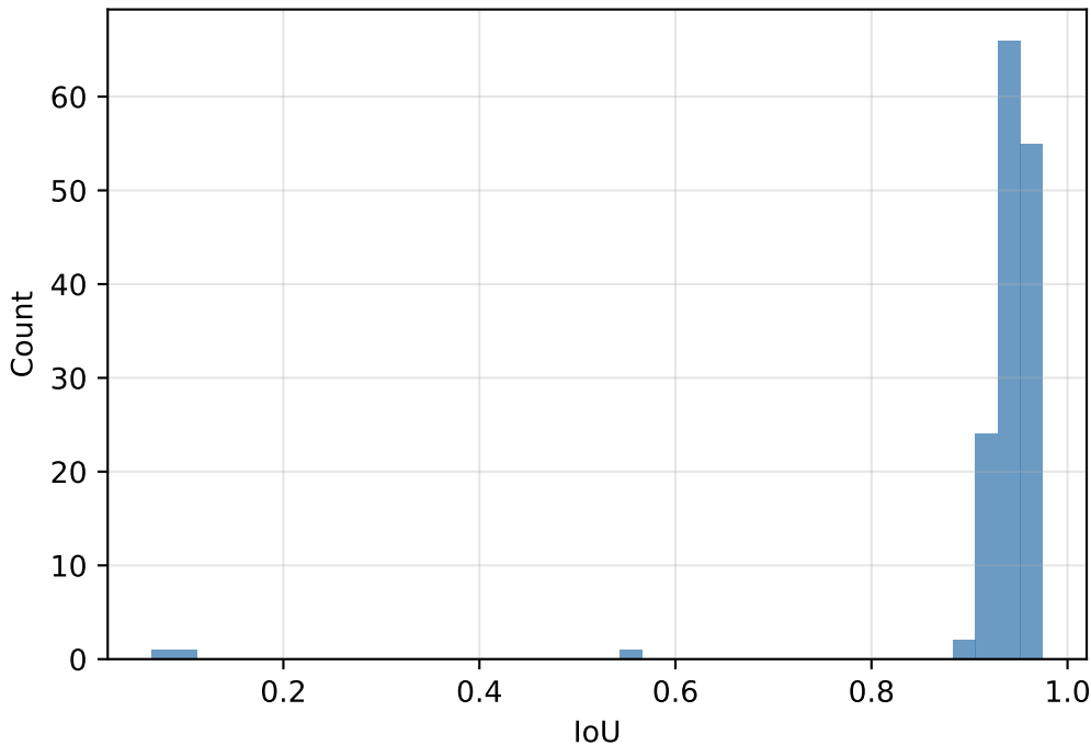
IoU Distribution
