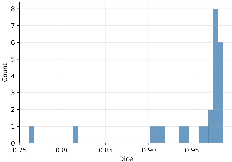
Dice Distribution
