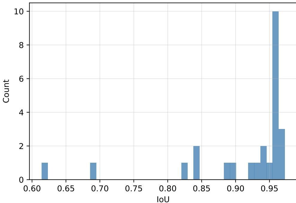
IoU Distribution
