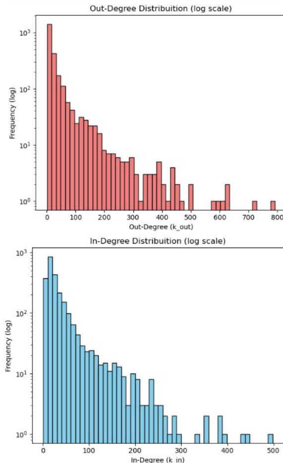
Figure 4. In and Out degree distribution from the created subset.
