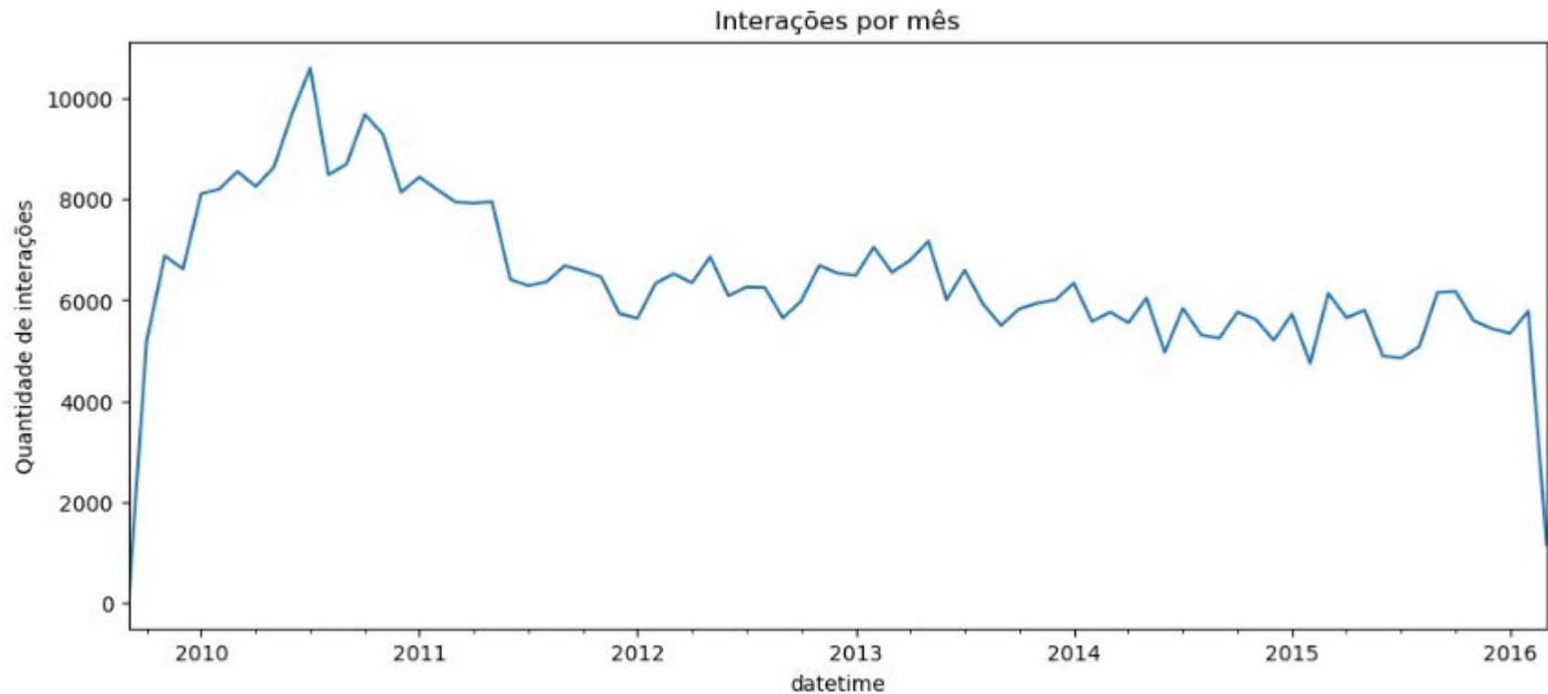
Figure 2. Temporal evolution of the volume of interactions (edges) in the Math Overflow dataset. The graph clearly shows a spike in growth between 2010 and 2011.
