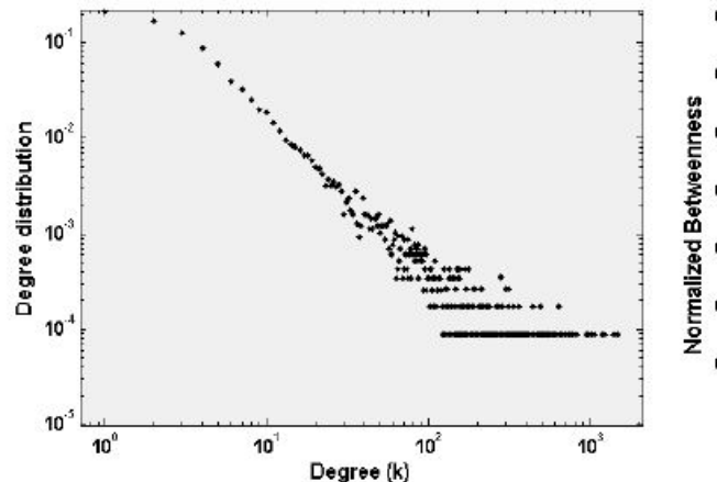
Figure 1. Heavy-tailed degree distribution in the MathOverflow network (Montoya et al., 2013).
