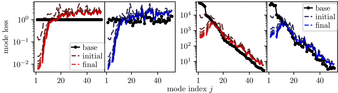
C) weighted train loss \sigma_j^2 L_j
