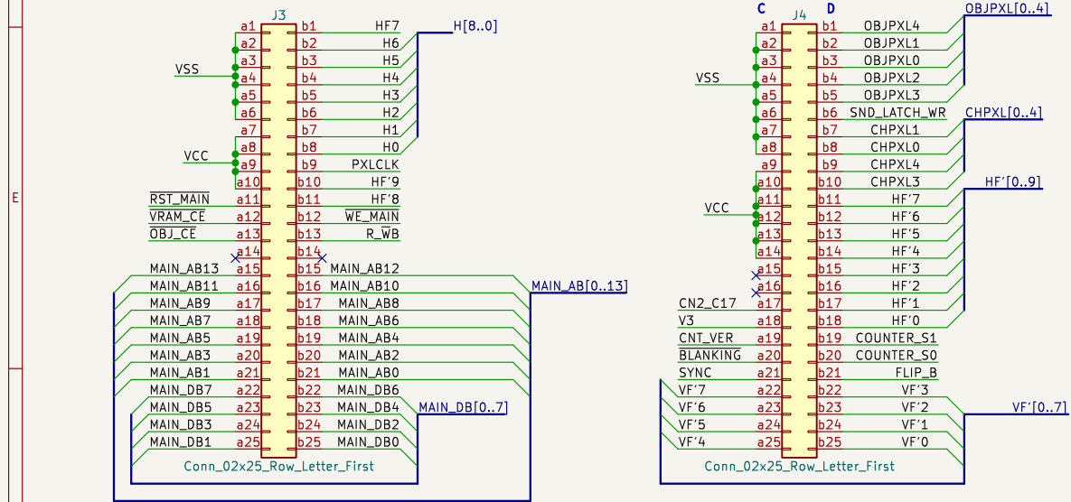
Bottom board connectors
