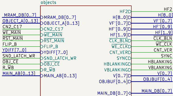
File: objects.kicad_sch
