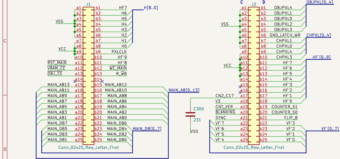
Top board connectors
