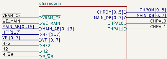
File: characters.kicad_sch
