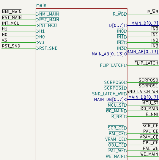
File: main.kicad_sch
