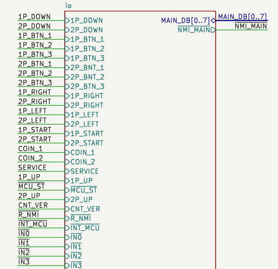
File: io.kicad_sch
