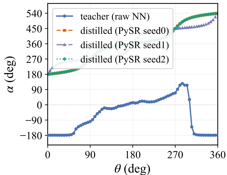
SAC seed1
