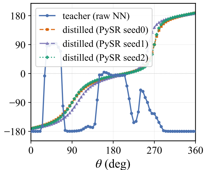
SAC seed0
