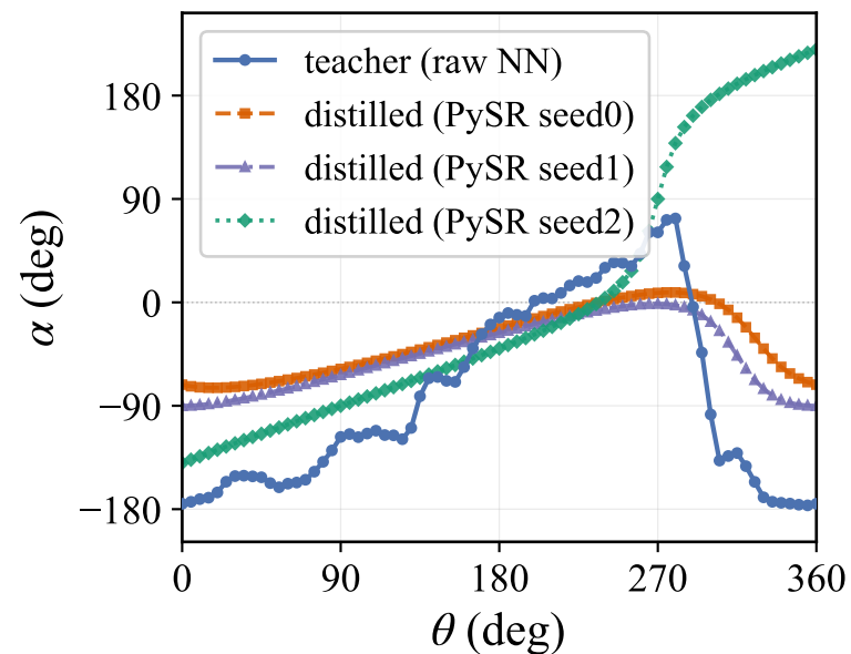
SAC seed2
