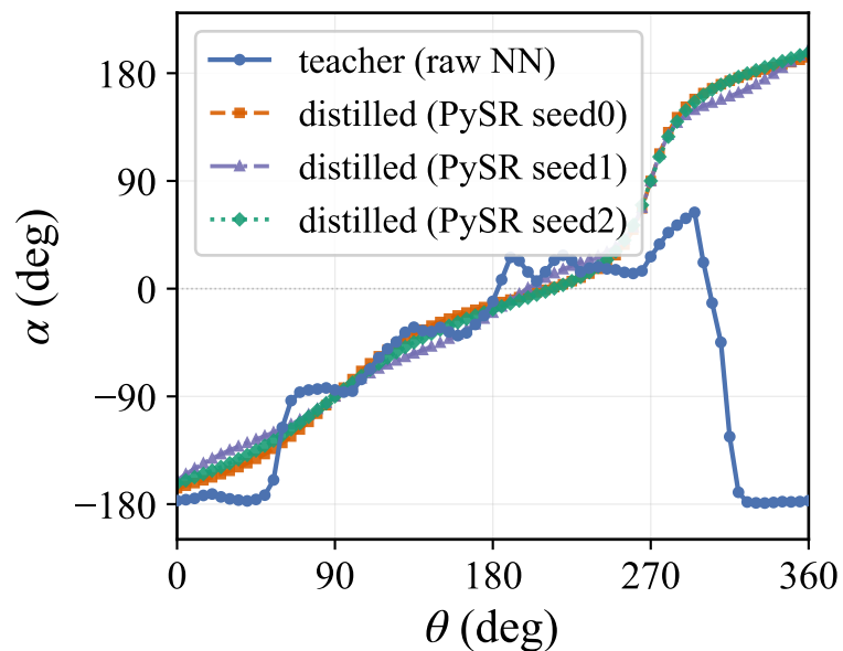
SAC seed4
