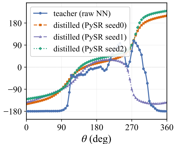
SAC seed3
