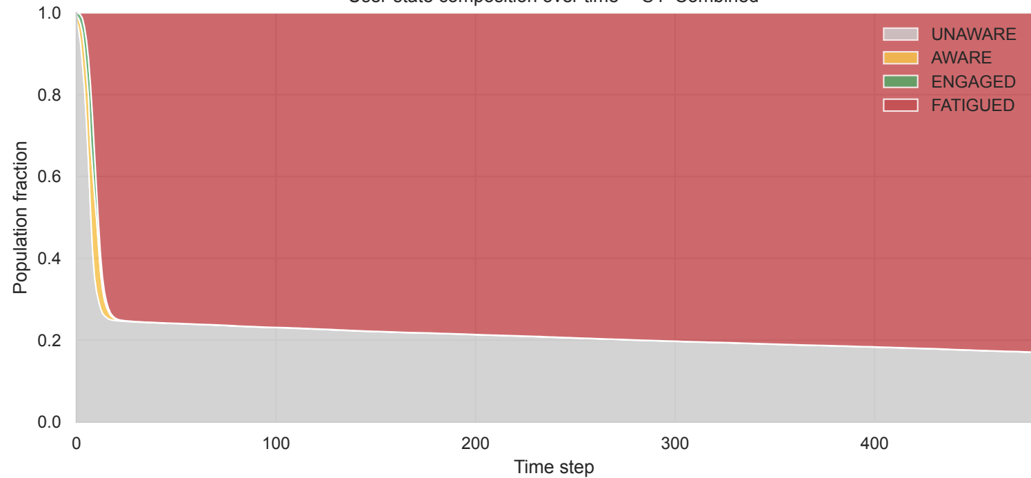
User-state composition over time -- S4 Combined
