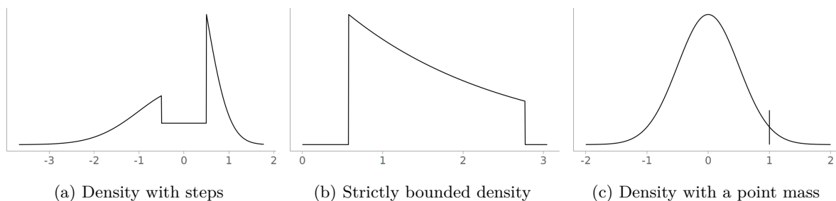
Figure 15: True densities for the examples used in Section 7.3, Section 7.4, and Section 7.5. Each of these examples poses a challenge for KDE density plots and histograms, and avoiding misrepresenting the data requires special attention.
